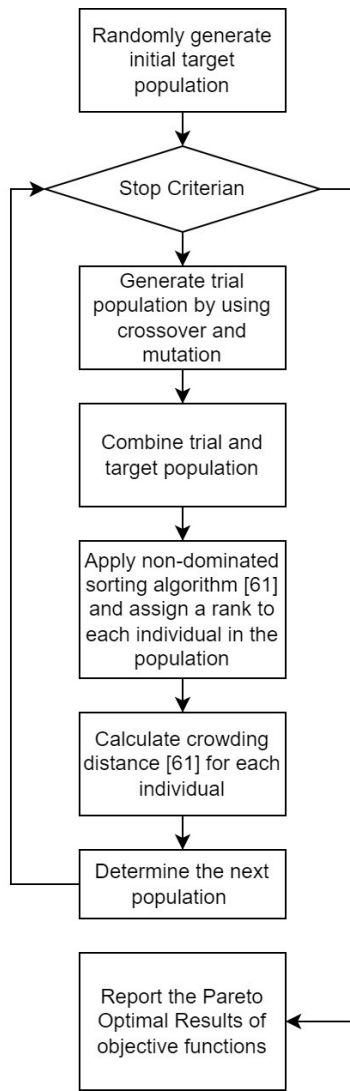
Fig. 7. Overview of the JDEMO algorithm flowchart.
