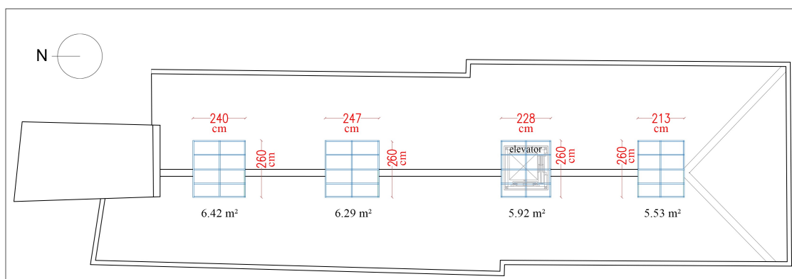
Fig. 3. Skylight measurements of historical akin passage.
