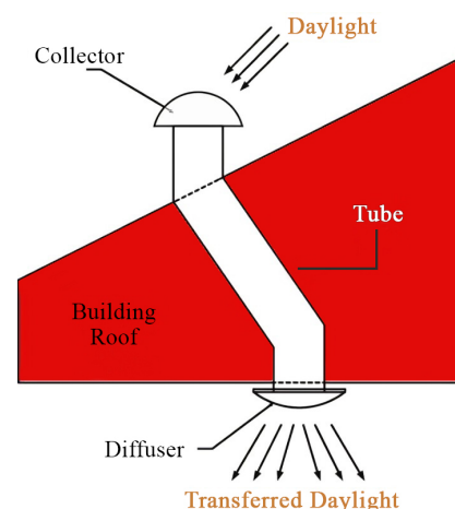
Fig. 1. Tubular Daylight Guidance System components (Source: Authors).
