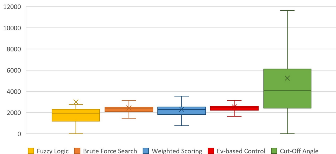
Fig. 7. Distribution of hourly maximum Ev (lux) during occupied hours throughout the year (The cross marker (x) indicates the average peak Ev for each control strategy).
