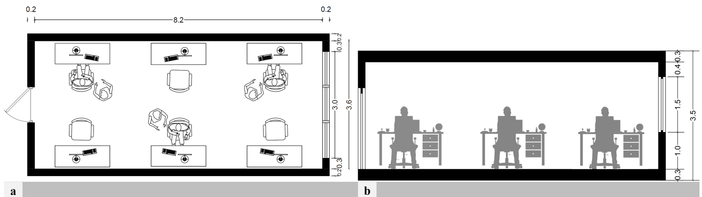
Fig. 4. Reference room: (a) plan and (b) section.
