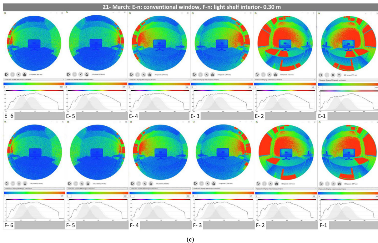
Fig. 13. (a)-(c) Performance of the light shelf with a depth of 0.30 m and the base case on the South orientation.
