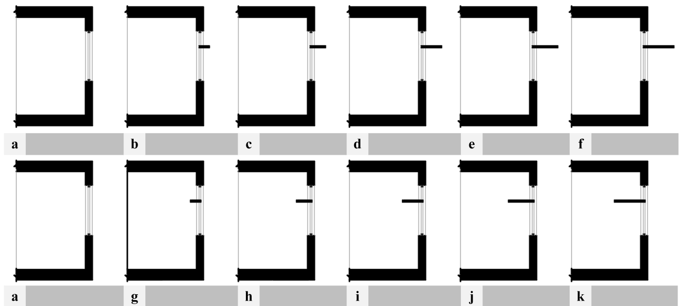
Fig. 5. Light shelves' configurations: exterior (a-f): a: base case, b: 0.30 m, c: 0.45m, d: 0.60m, e: 0.75m, f: 0.90m / Interior (a-k): a: base model, g: 0.30m, h: 0.45m, i: 0.60m, j: 0.75m, k: 0.90m.
